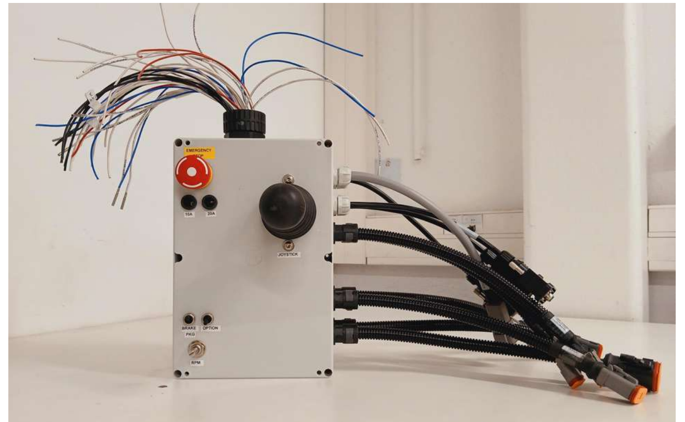
Wiring and box integration for construction and handling vehicles
